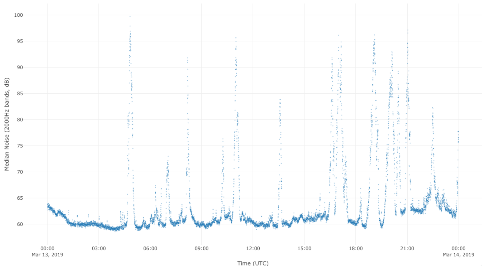
Noise Over Time for 13 March 2019
